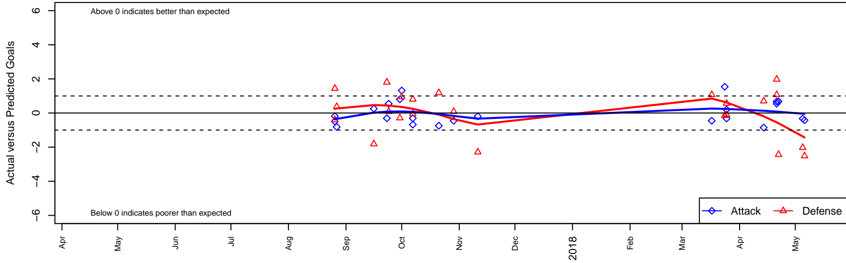
Wenatchee FC G05 Dots are actual minus expected GF (blue circles) and GA (red triangles). Blue line is smoothed change in attack strength. Red is smoothed change in defense strength.
